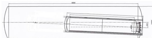
Figur 1 Ammonia pressure tank integrated in the slurry tanker
